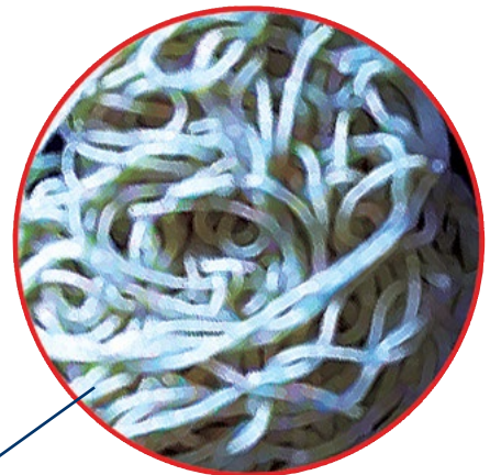
Amorphous
