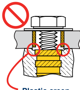
Plastic creep
